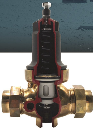
CYCLE GARD ® CONSTANT PRESSURE PUMP CONTROL
